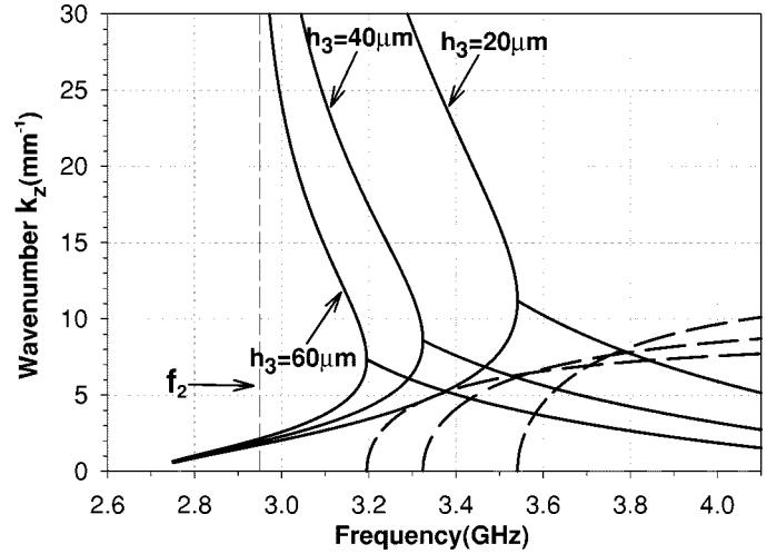
Fig. 3. Dispersion curves for the propagation constant of the first magnetostatic mode of the structure in Fig. 1 with h_1 = h_4 \rightarrow \infty , h_2 = 100 \mu\text{m} , w = 1 mm, \phi = 0 , \mu_0 H_0 = 0.0632 T, and \mu_0 M_s = 0.0840 T. Curves are plotted for h_3 = 20, 40, 60 \mu\text{m} . Solid lines: phase constant ( \text{Re}(k_z) ). Dashed lines: attenuation constant ( |\text{Im}(k_z)| ).
